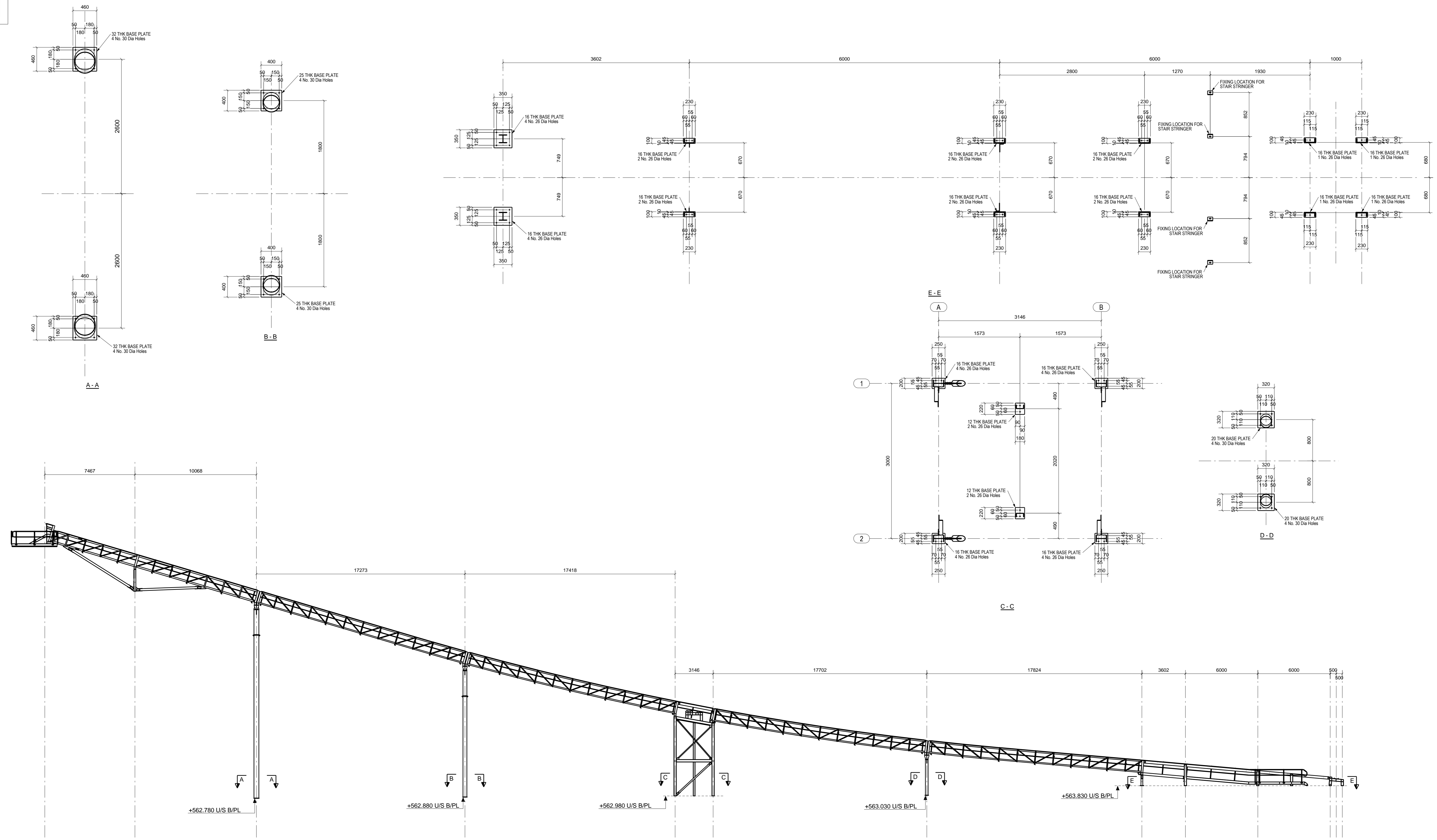
ELEVATION ON View_02 (PLAN +562780)
